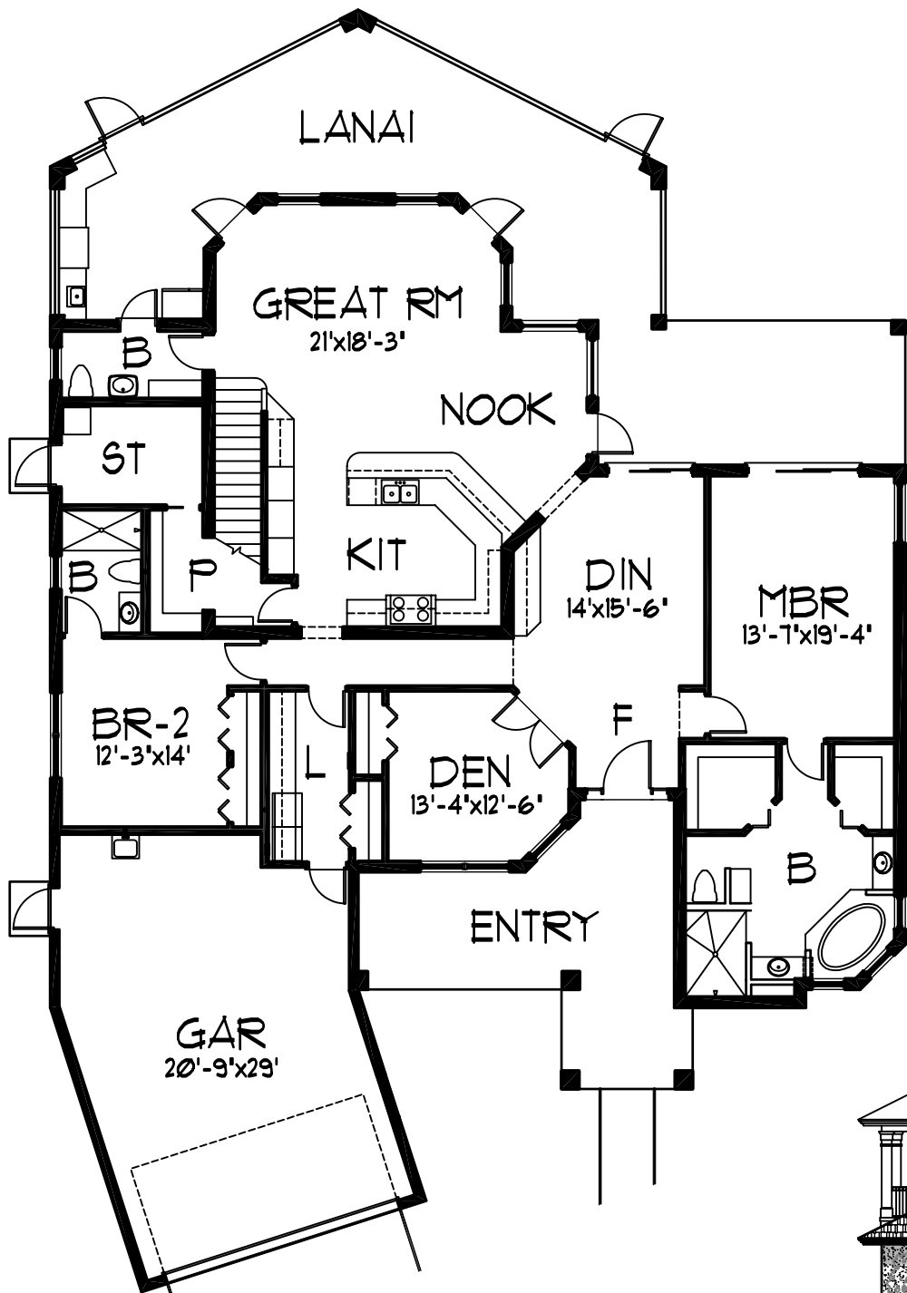
FIRST FLOOR PLAN 2580 S.F. TOTAL LIVING: 3326 S.F.
