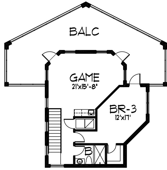
SECOND FLOOR PLAN 746 S.F.
