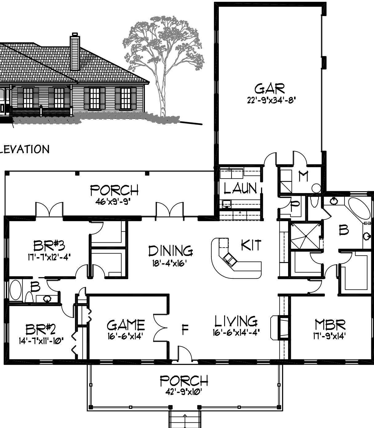
FIRST FLOOR PLAN TOTAL LIVING: 2923 S.F.
