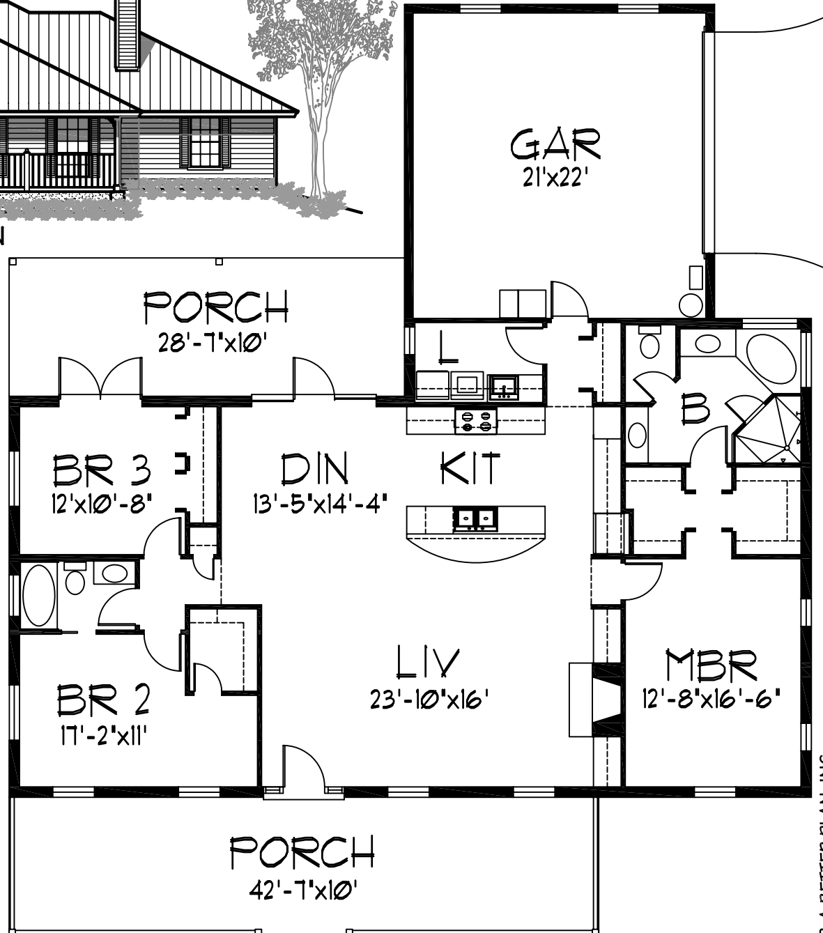
FLOOR PLAN TOTAL LIVING: 1842 S.F.
