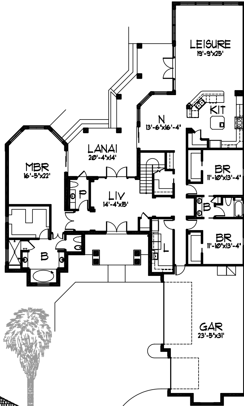
FIRST FLOOR PLAN TOTAL LIVING: 4257 S.F.
